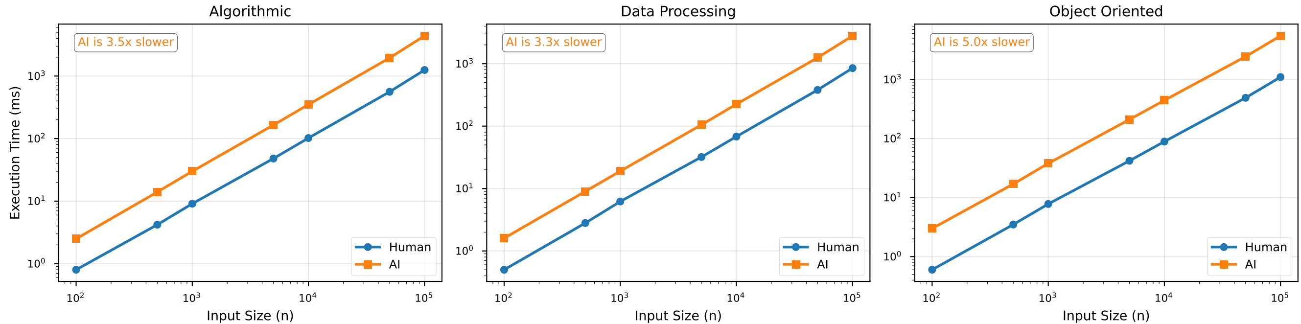
Figure 3.1: Performance Scaling with Input Size (Log-Log Plot)
